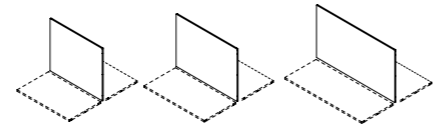
Pannello divisorio frontale/ Frontal panel L 80/100/120 P 2,5 H 60
